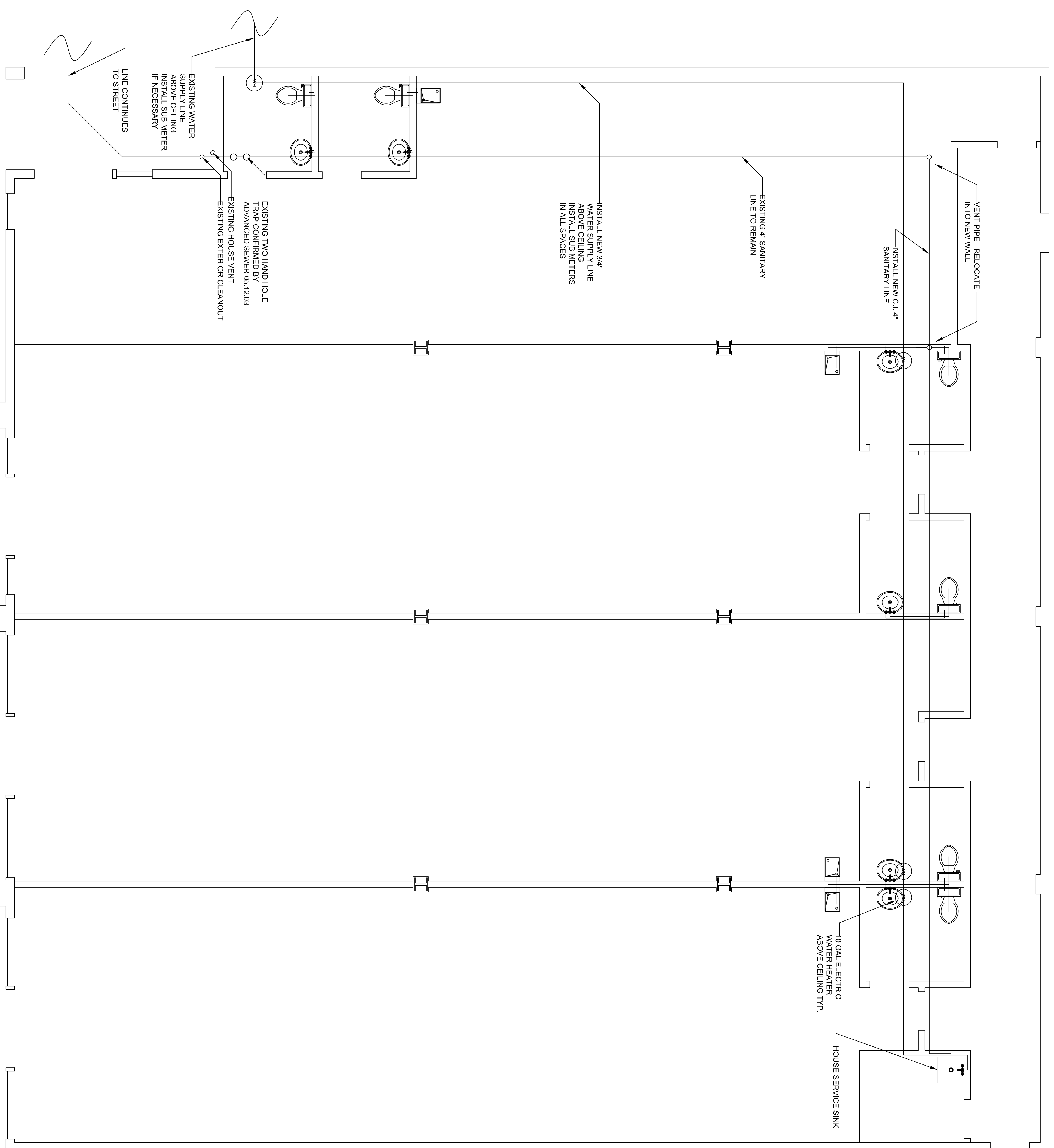
PLUMBING PLAN SCALE: 1/4" = 1'
